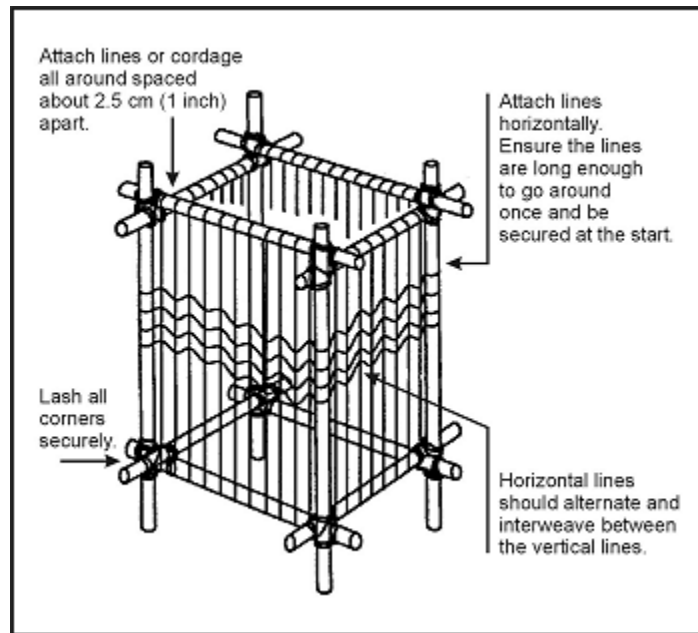
Figure 12-10. Square Pack
