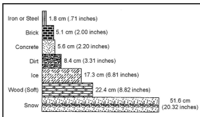
Figure 23-1. Materials to Reduce Gamma Radiation
