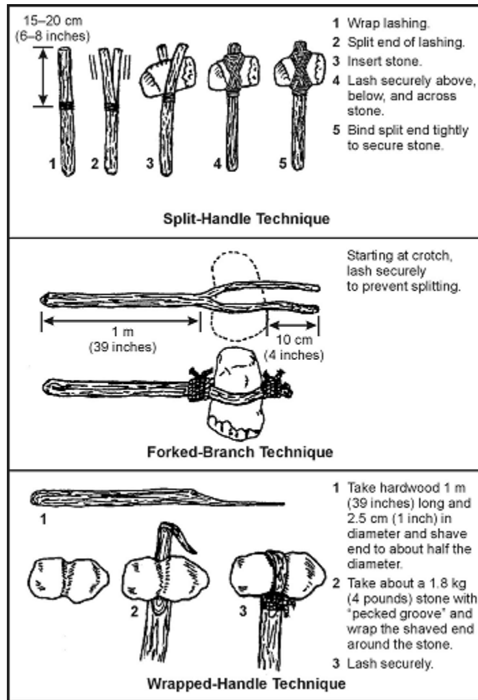
Figure 12-1. Lashing Clubs
