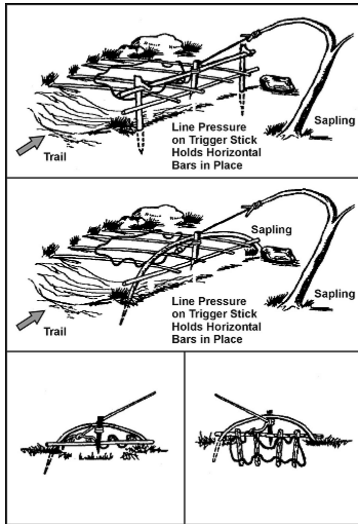
Figure 8-12. Treadle Spring Snare
