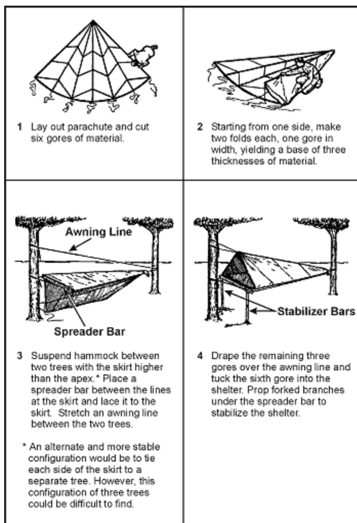
Figure 5-8. Parachute Hammock
