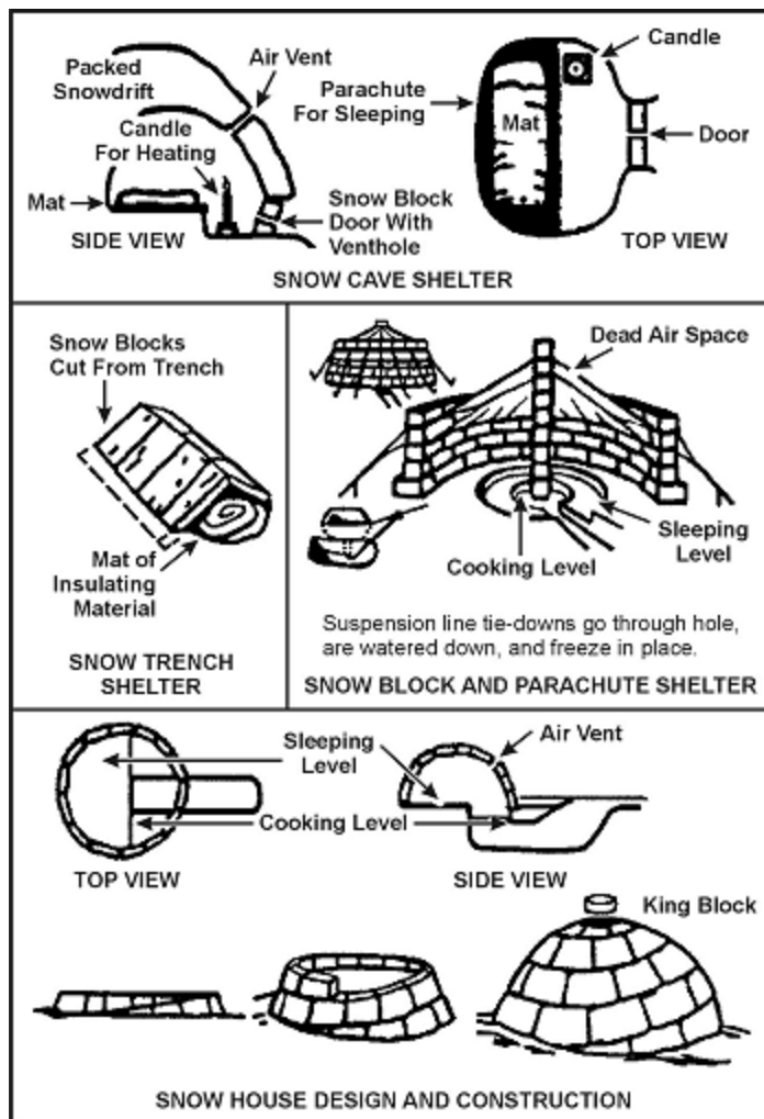
Figure 15-4. Snow Dwellings
